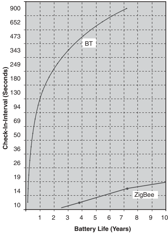
Figure 2.4 Battery longevity. (From [2.32].)
