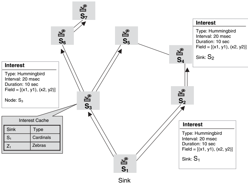
Figure 6.12 Interest propagation.
