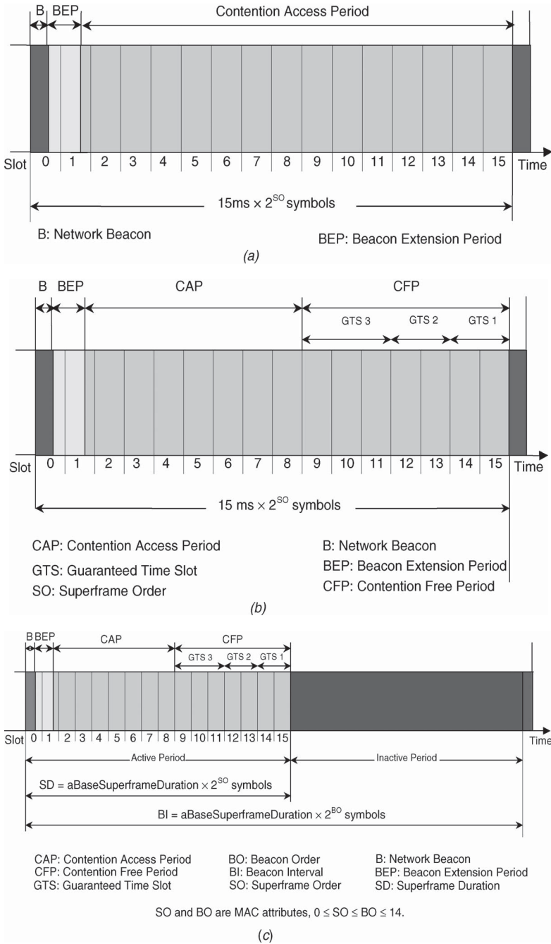
Figure 5.16 (a) Superframe structure; (b) QoS frame structure; (c) Superframe structure with energy saving.
