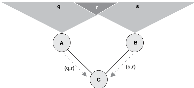
Figure 6.5 Flooding traffic overlapping problem.
