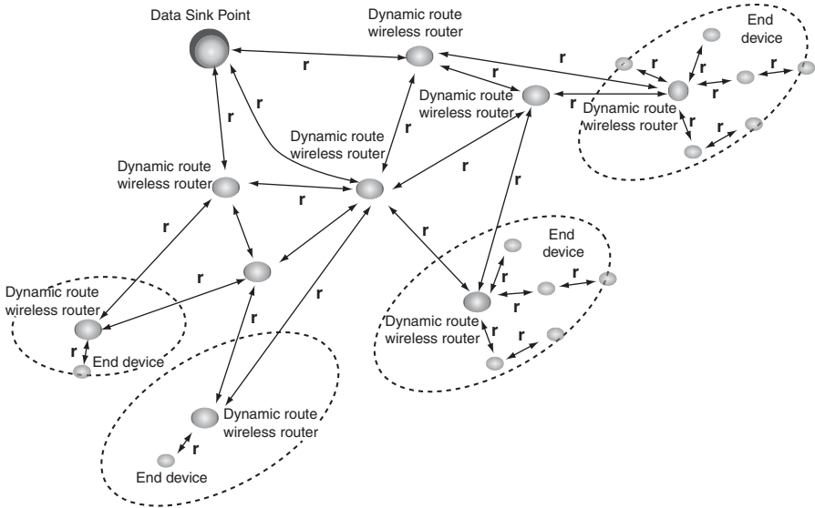
Figure 2.2 Category 1 WSNs: multipoint-to-point, multihop systems utilizing dynamic routing.
