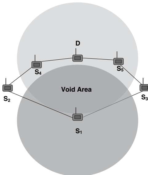
Figure 6.17 Greedy algorithm forward progress failure.
