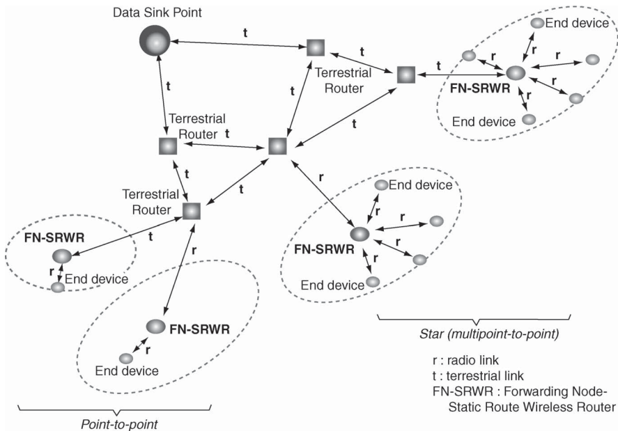
Figure 2.1 Category 2 WSNs: point-to-point, generally-singlehop systems utilizing static routing.
