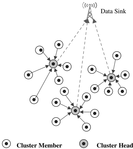
Figure 6.9 LEACH network model.
