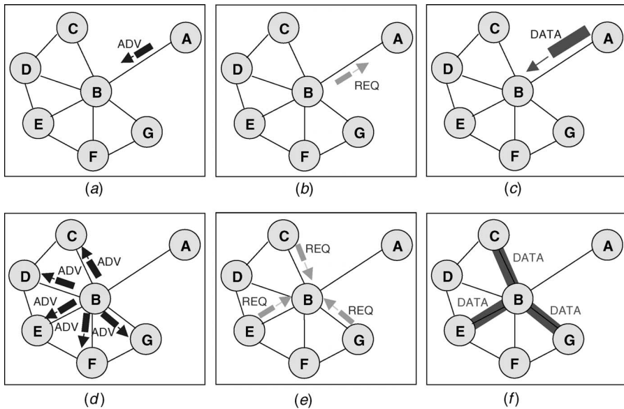
Figure 6.6 SPIN basic protocol operations [6.17].
