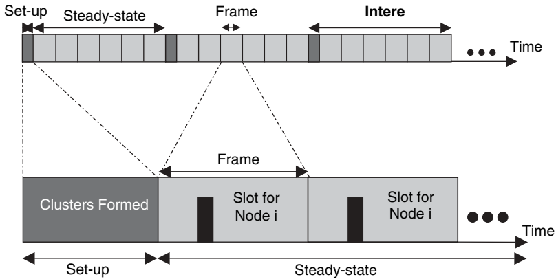
Figure 6.10 LEACH phases [6.18].
