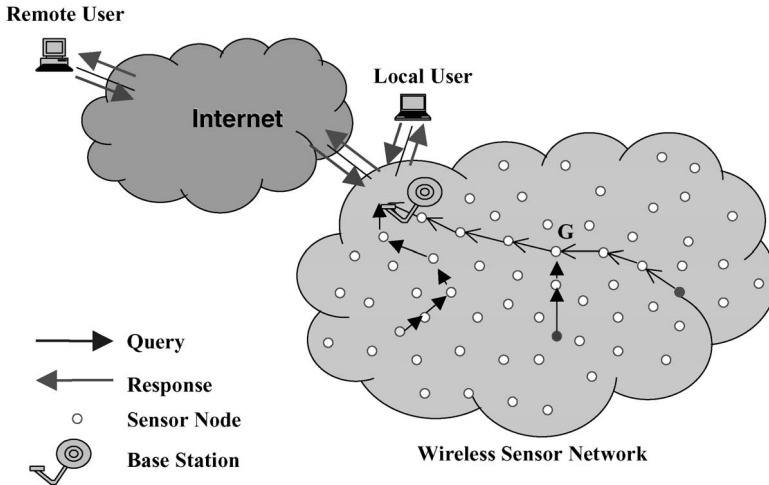
Figure 6.2 Multihop data and query forwarding.
