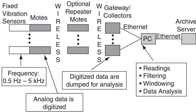
Figure 2.11 Intel fab environment with WSNs.
