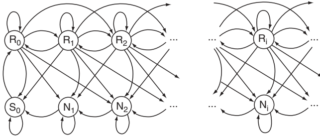
Figure 11.4 DTMC sensor node model. (From [11.17].)
