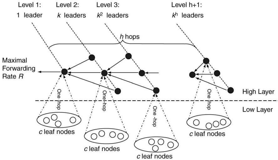
Figure 11.6 Two-tiered topology of a WSN.
