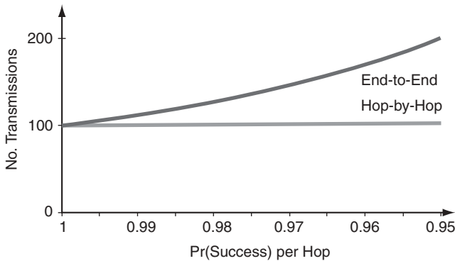
Figure 7.2 Hop-by-hop versus end-to-end: number of transmissions required to send 10 packets in 10 hops. (From [7.3].)
