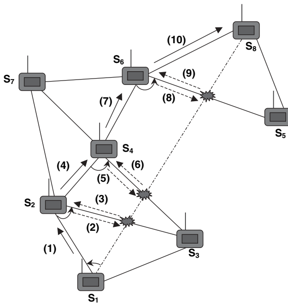
Figure 6.18 Perimeter traversal on a planner graph.
