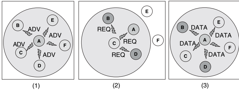
Figure 6.8 SPIN-BC protocol basic operations [6.17].
