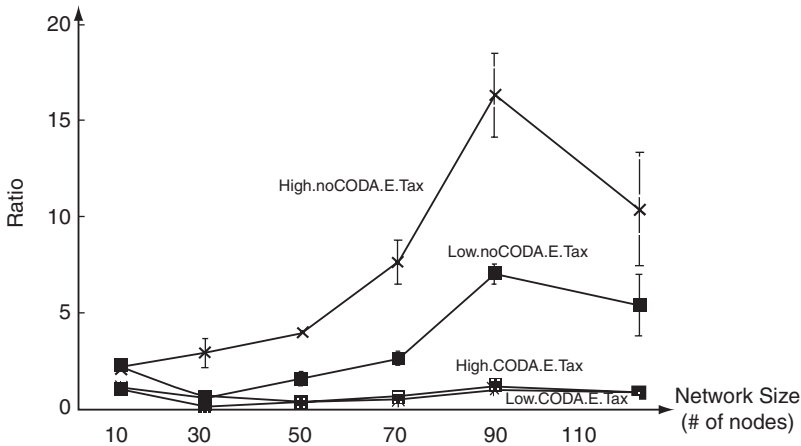
Figure 7.1 Energy tax in CODA as a function of network size for high- and low-data-rate traffic. The difference between the data points with and without CODA indicates the energy saving achieved by CODA. (Based on data from [7.1].)
