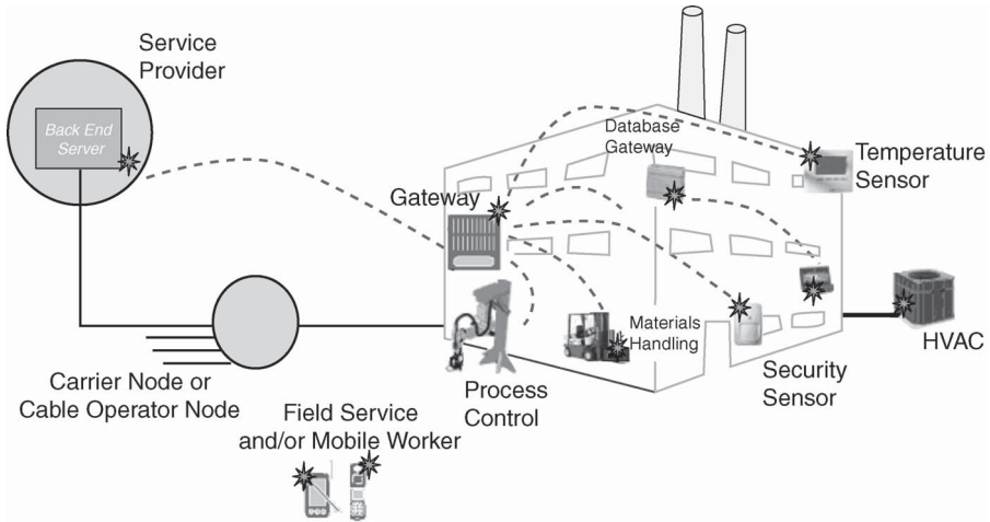
Figure 2.7 Industrial control applications.
