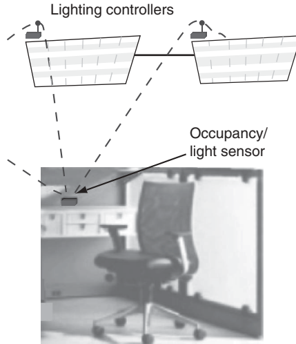
Figure 2.6 Indoor lighting control.
