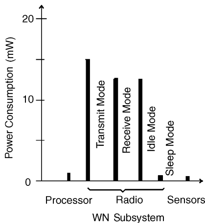
Figure 11.3 Energy consumption for each subsystem in sensor nodes. (From [11.7].)
