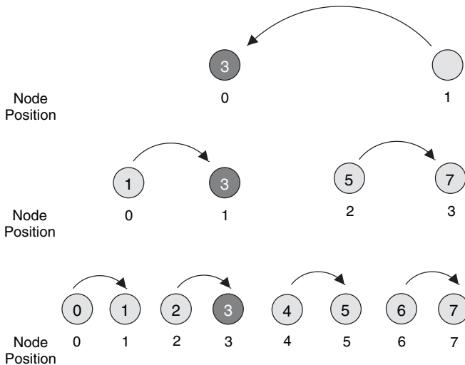
Figure 6.11 Chain-based data gathering and aggregation scheme [6.21].
